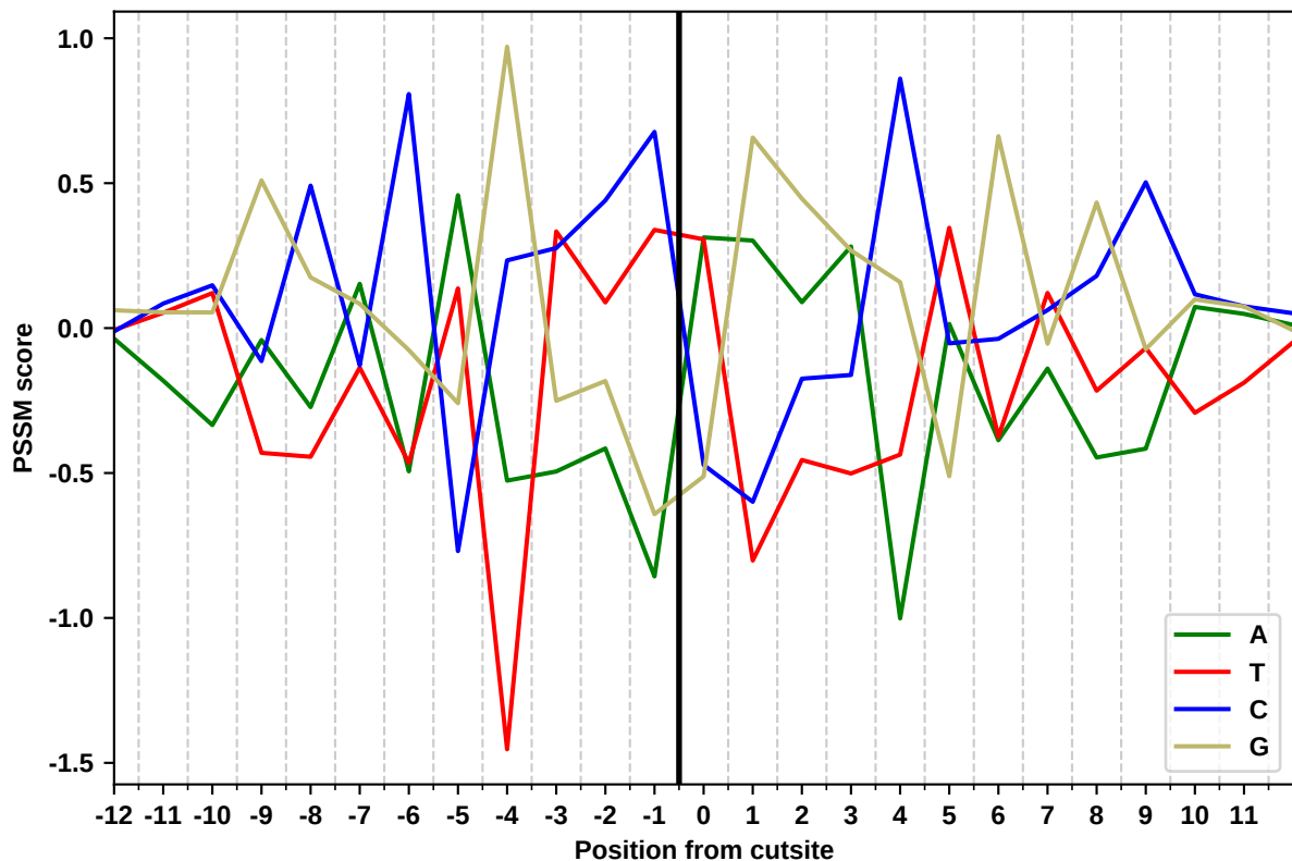
Tn5 insertion bias of reads (forward)
