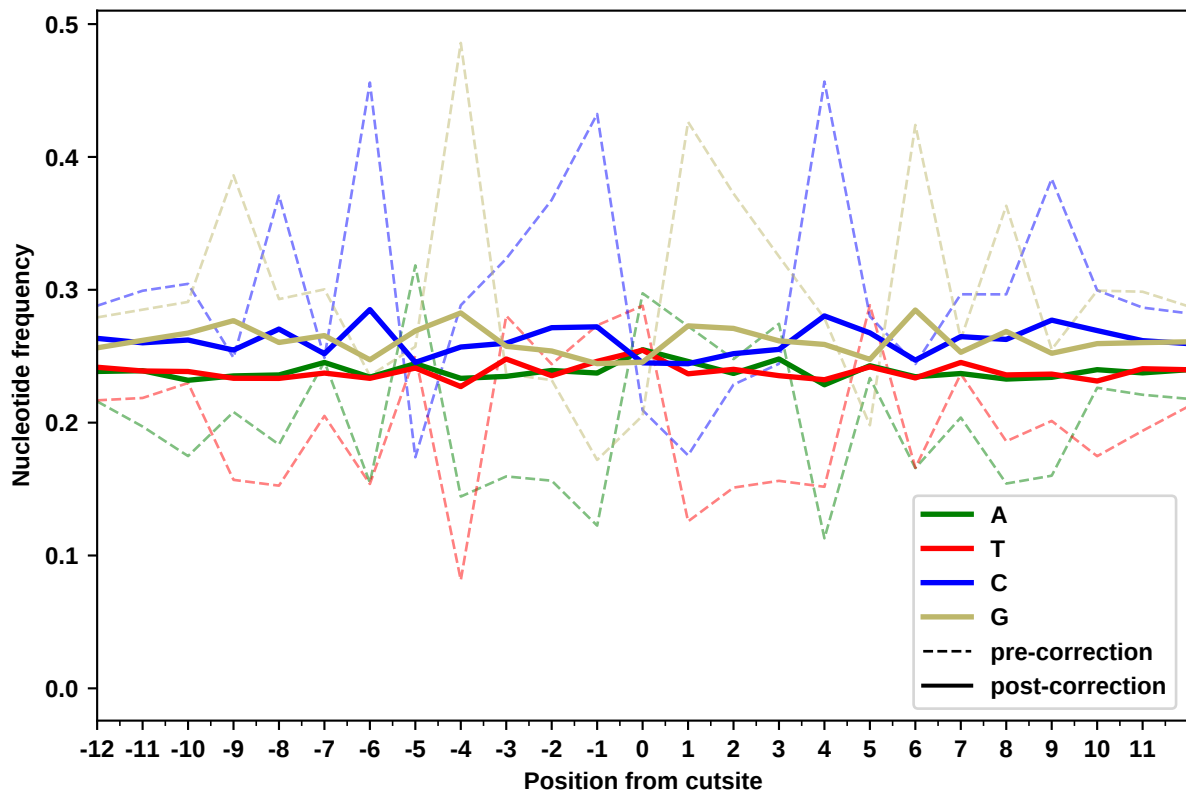
Nucleotide frequencies in corrected reads (forward strand)
