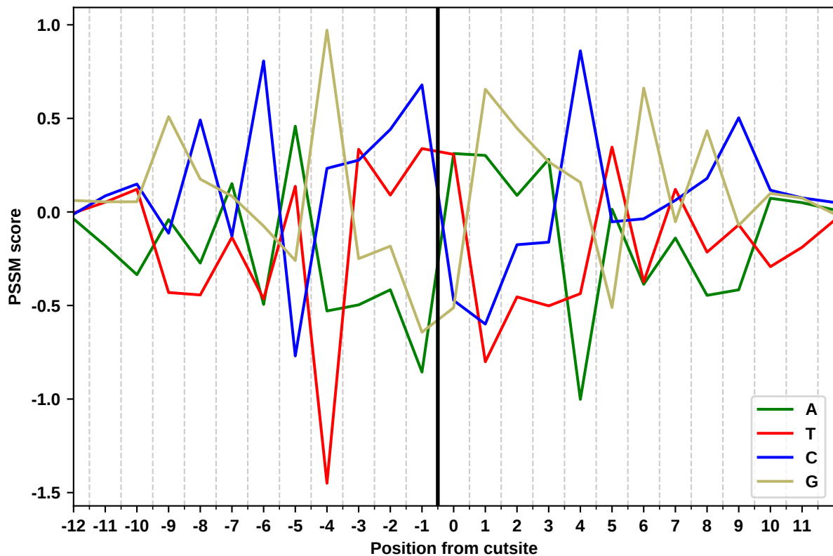
Tn5 insertion bias of reads (reverse)
