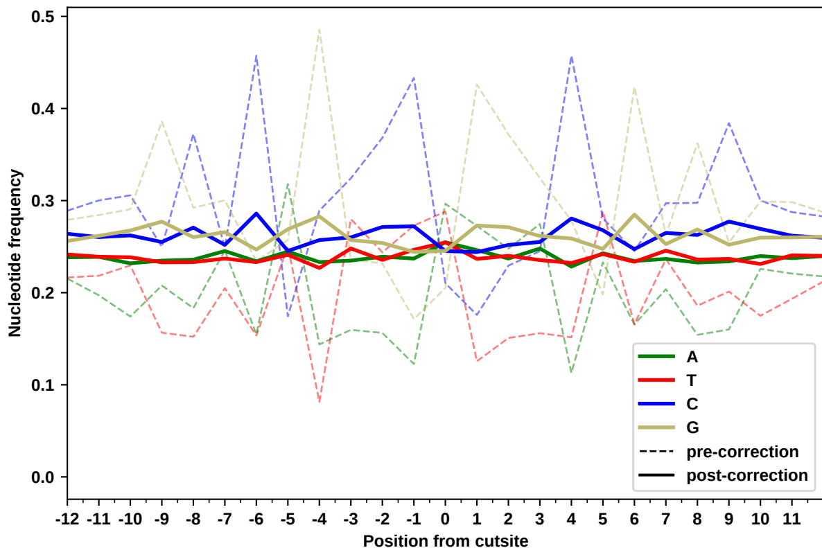
Nucleotide frequencies in corrected reads (reverse strand)
